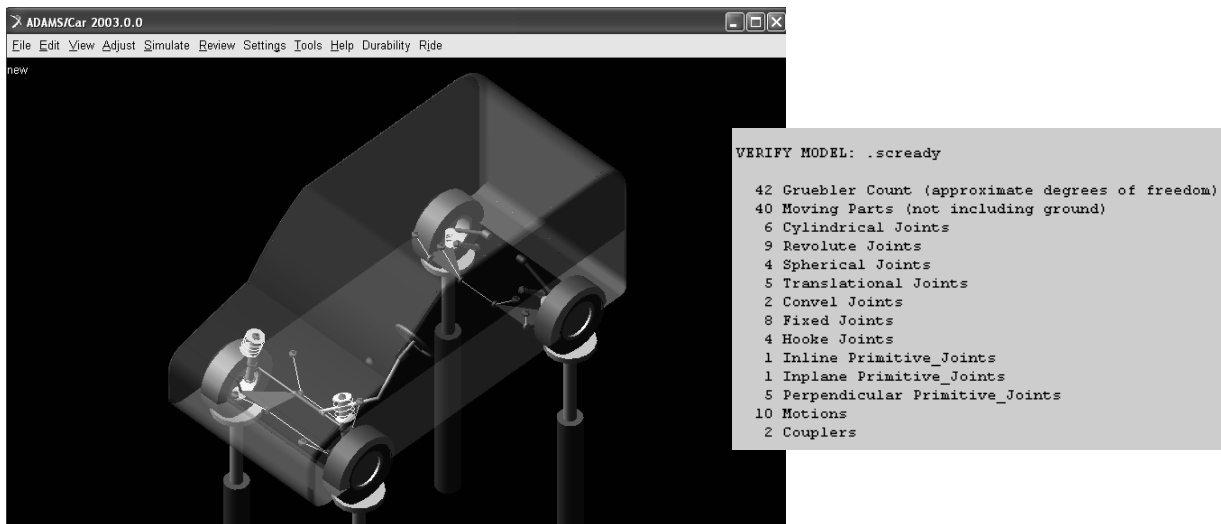
Fig. 6. The complete view of the vehicle on the test rig
