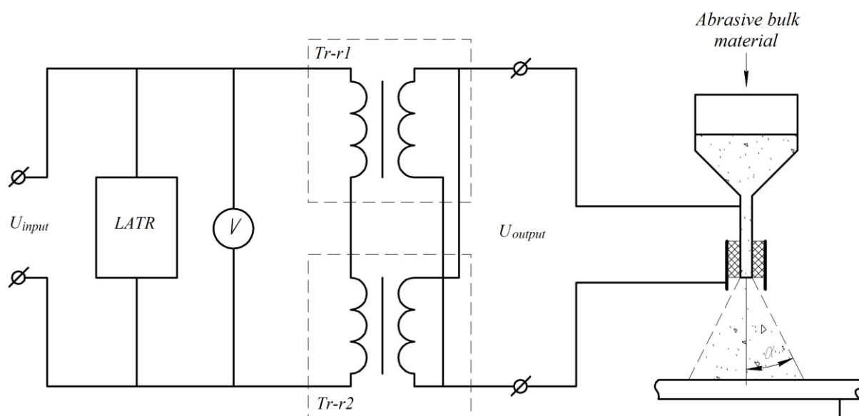
Fig. 1. The scheme of charging and the supply of abrasive particles on metal surfaces
