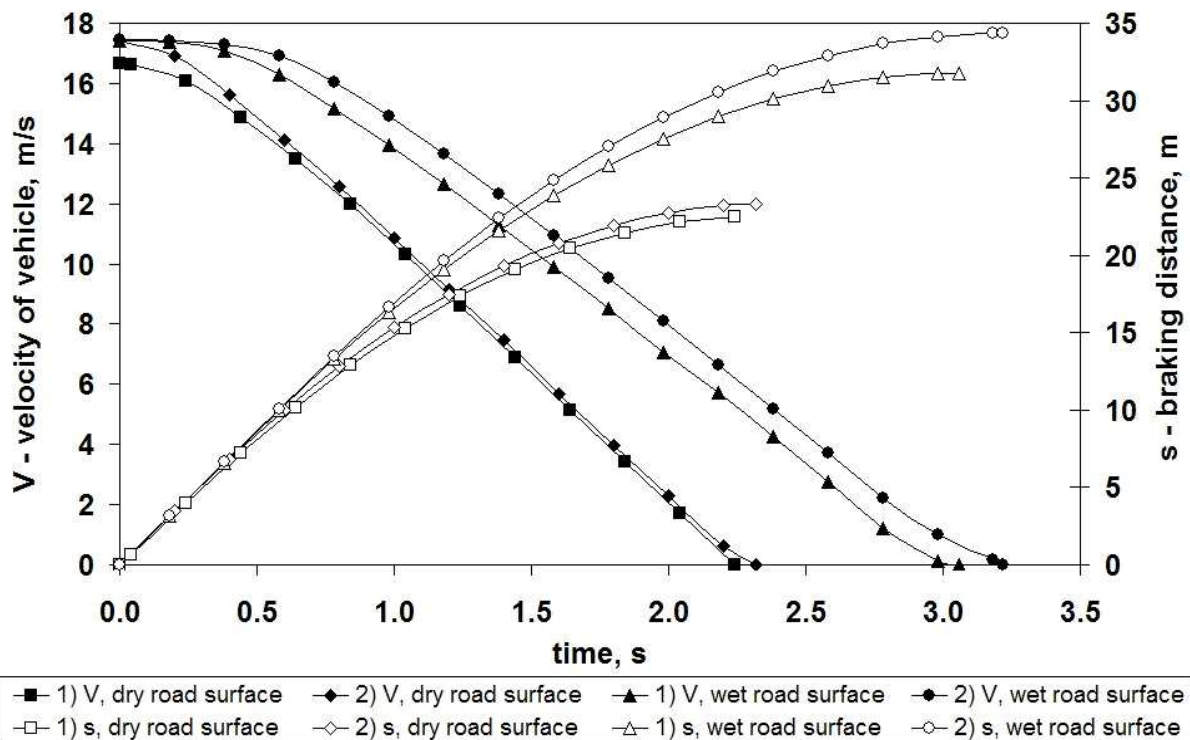
Fig. 9. The vehicle velocity and the braking distance in terms of braking time with too low pressure in tyres of front wheels
