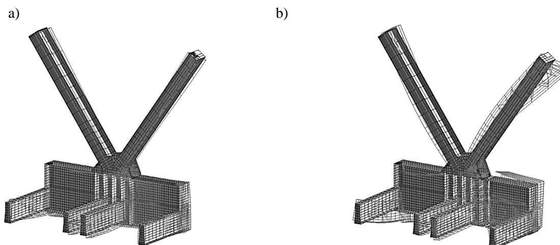
Fig. 2. View of the local disorder of vibration form (a horizontal flexural form, f=19.72\text{Hz} ) resulting from damage: a) node with no damage; b) node with damage
